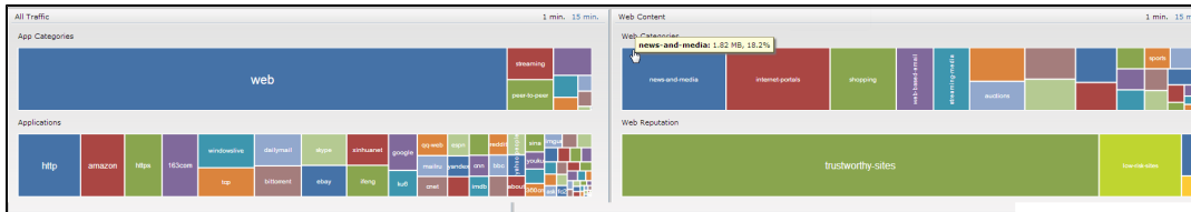
Figure 71 AppRF Dashboard
